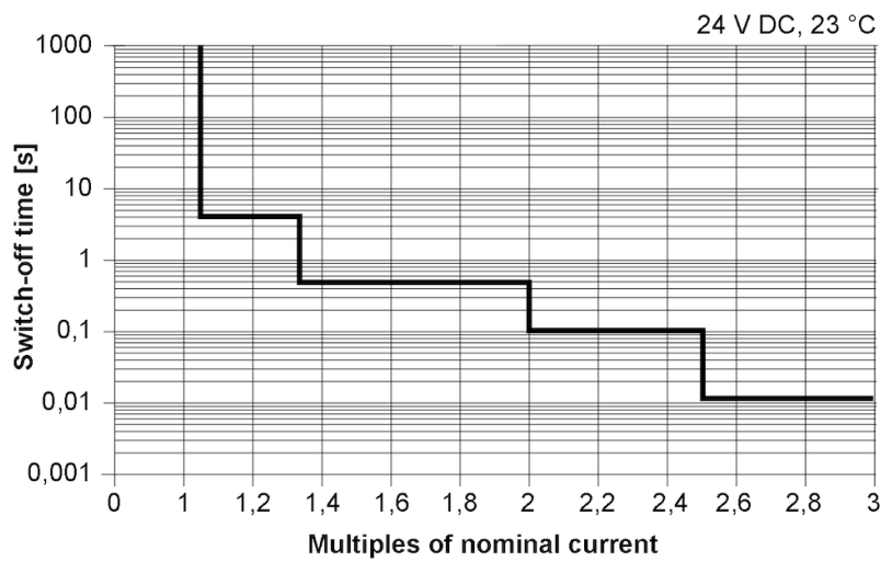
Time-current characteristics
