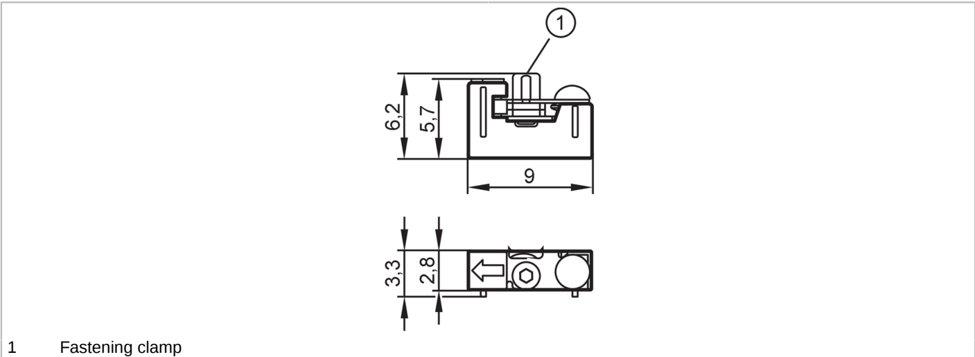
1 Fastening clamp
