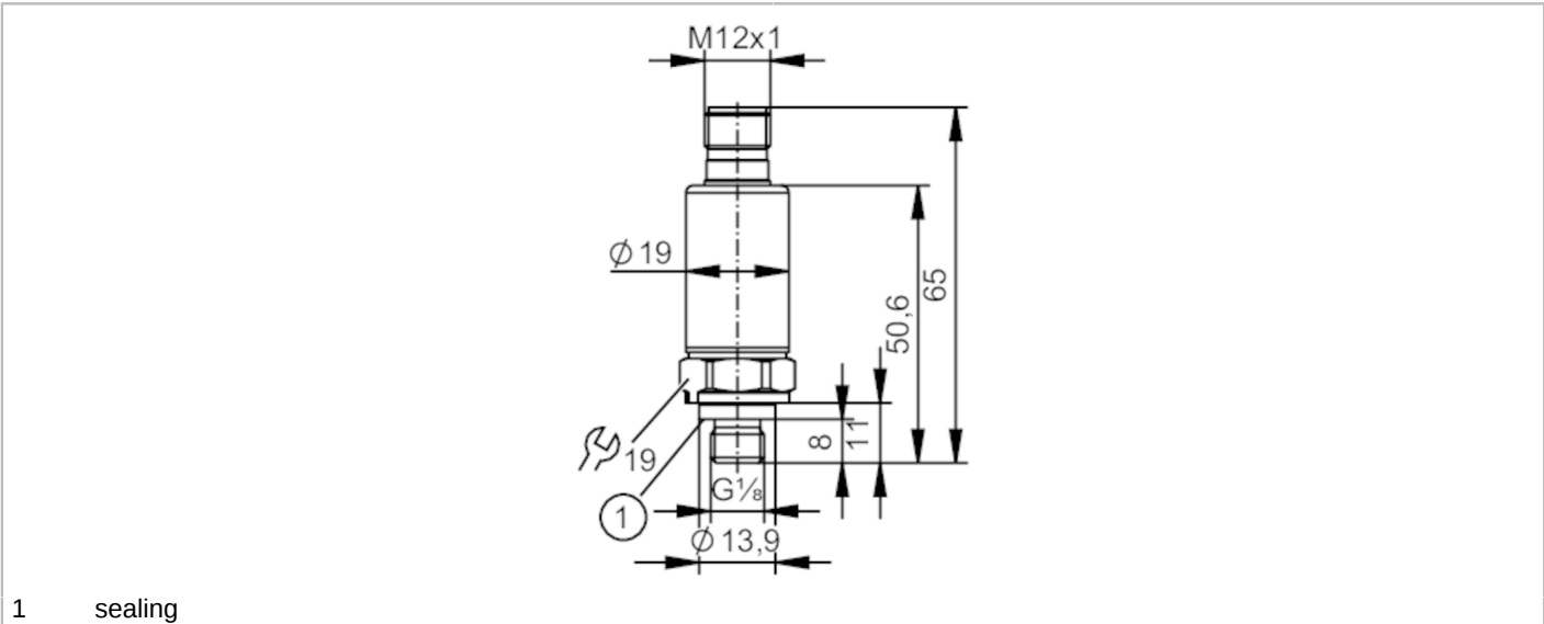
1 sealing
